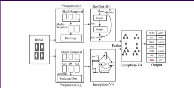
Figure 1: Intracranial hemorrhage detection model Asif et al.
